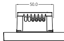
⑥ TOP VIEW
