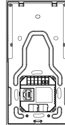
④ BACK VIEW
