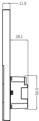
② RIGHT VIEW
