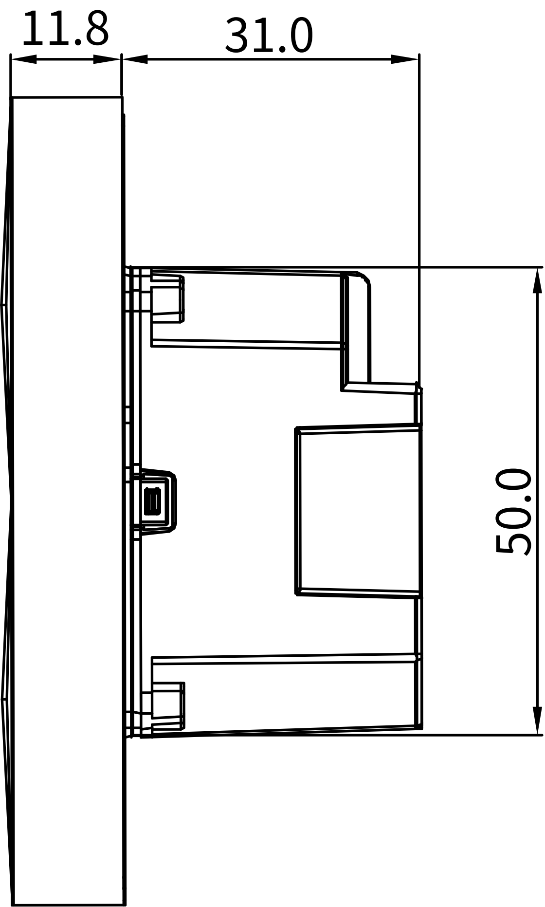
② RIGHT VIEW
