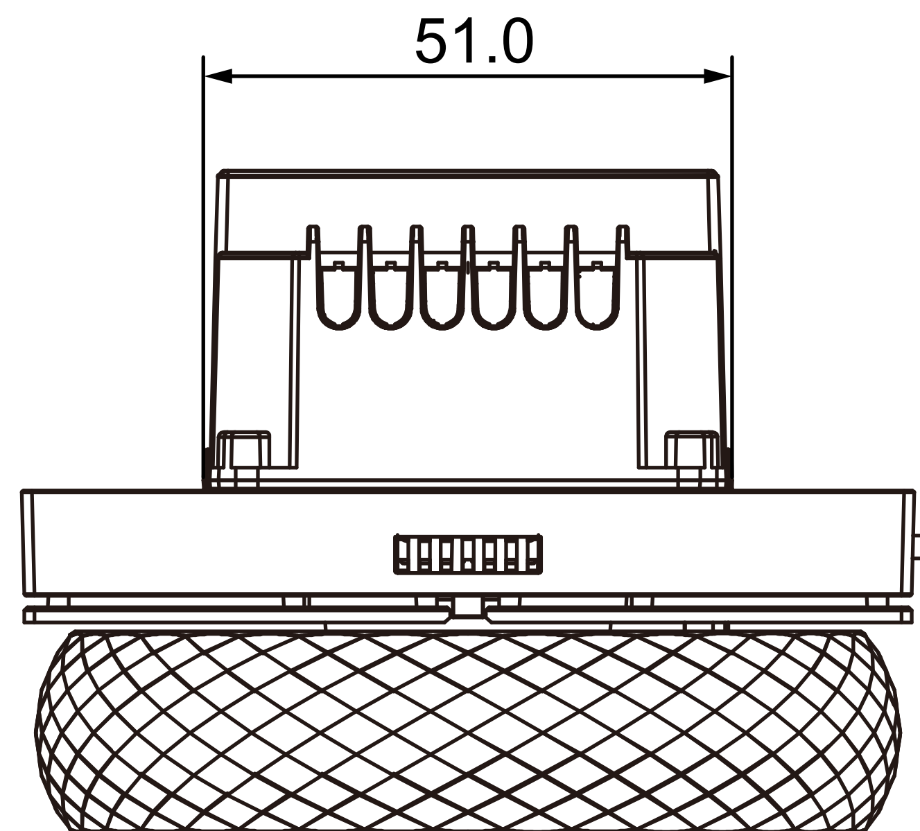
⑥ TOP VIEW
