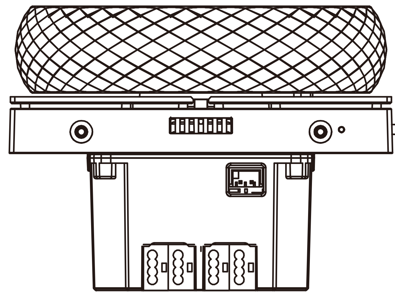
⑤ BOTTOM VIEW
