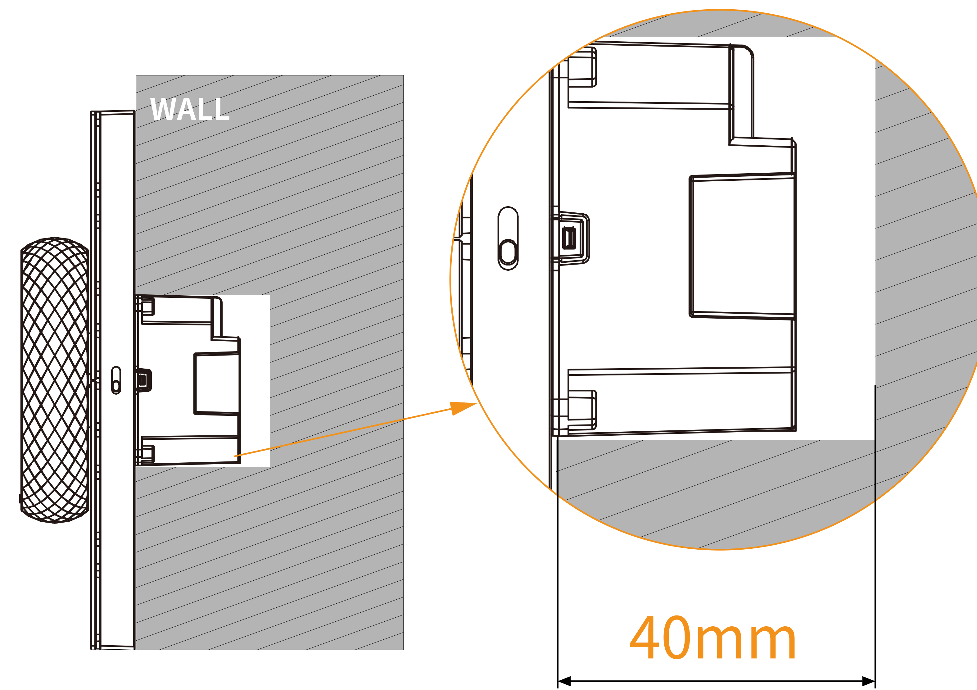
2 SIDE VIEW:HYPANEL LUX IN WALL
