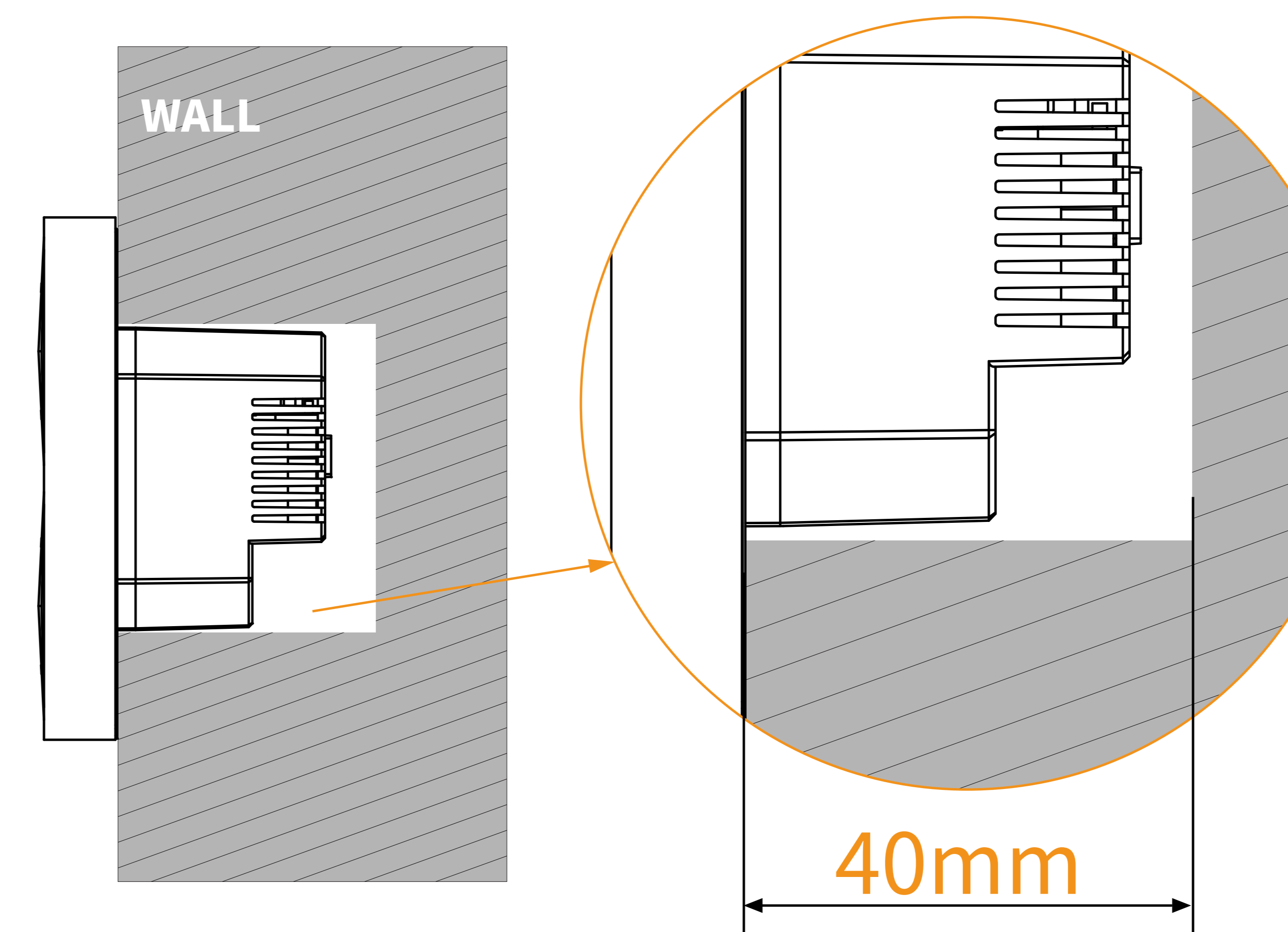
② SIDE VIEW:HYPANEL LITE IN WALL
