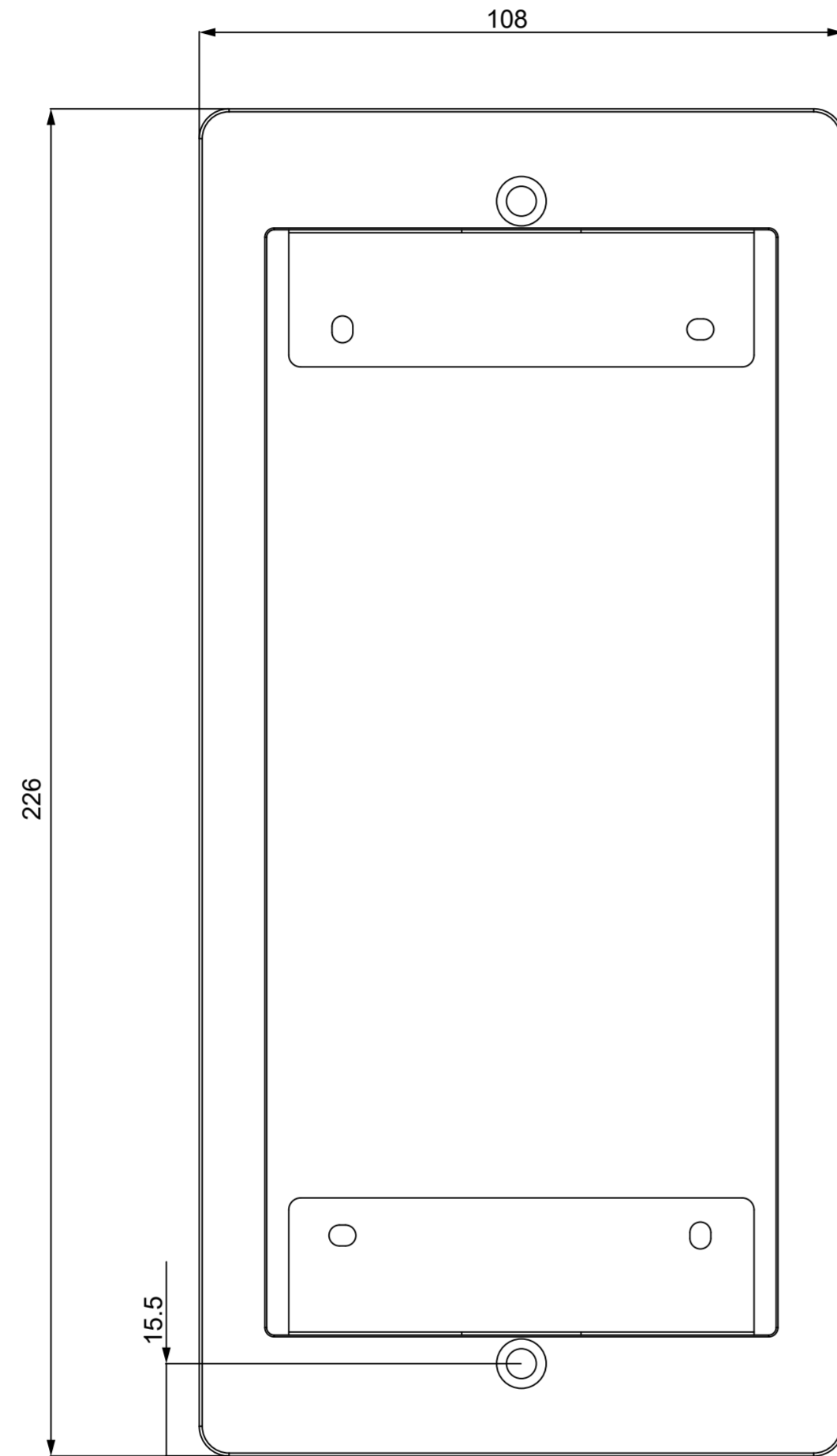
1 FRONT VIEW
