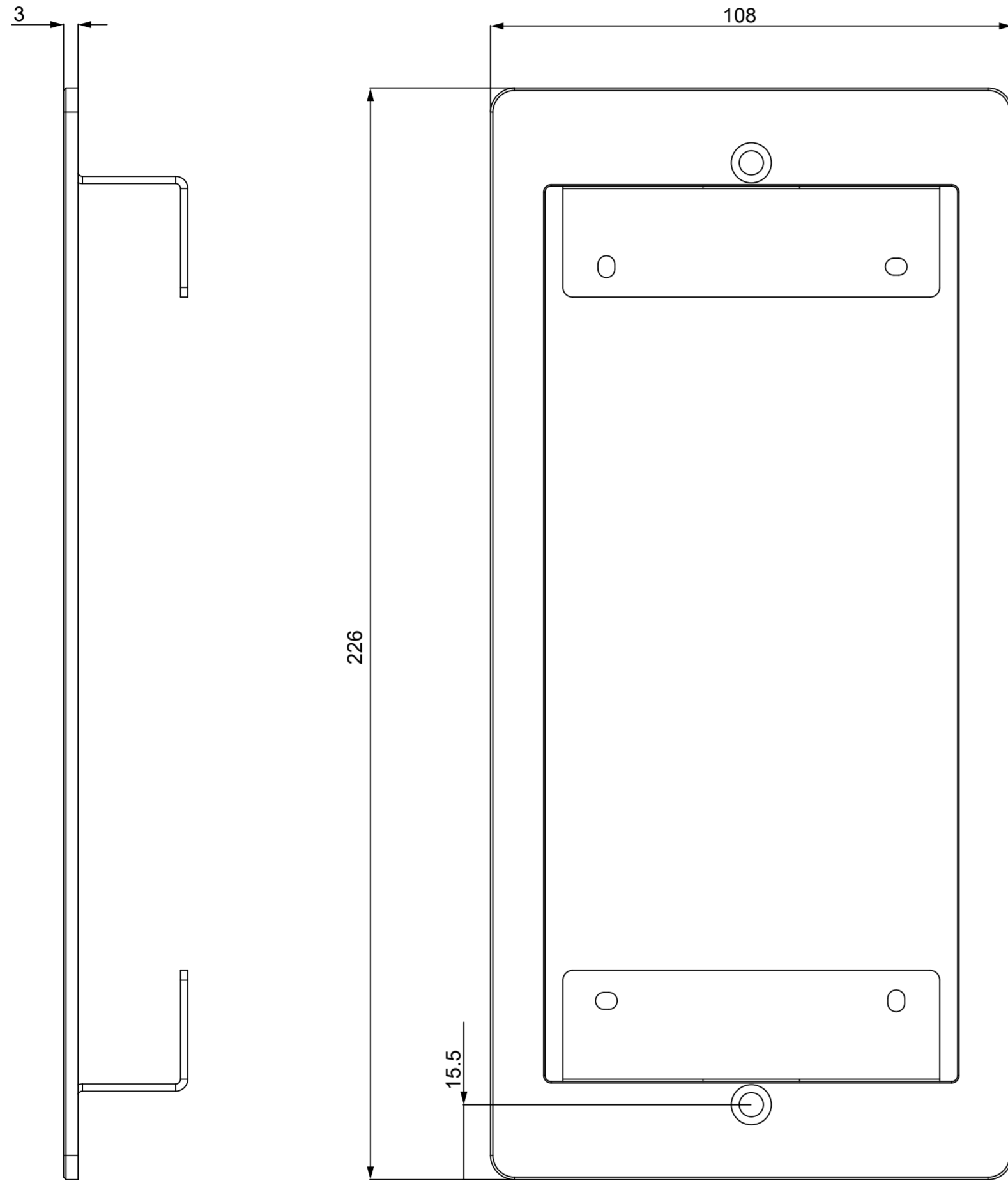
1 FRONT VIEW
